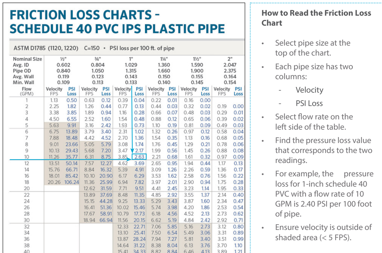
Figure 5-2: Friction loss chart for schedule 40 PVC (image courtesy of Hunter Industries Inc)
