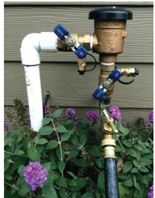
Figure 6-4: Backflow device.
