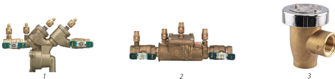
Figure 5-8: Left to right (1) RP double check valve, (2) double check valve, (3) atmospheric vacuum breaker (images courtesy of Watts)
