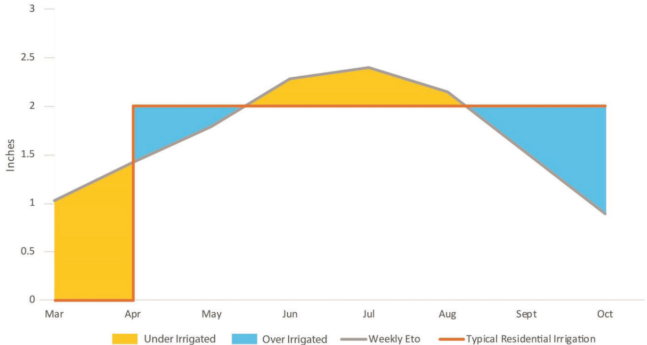
Figure 8-2: Weekly ETo for UNR Campus station vs. typical residential irrigation
