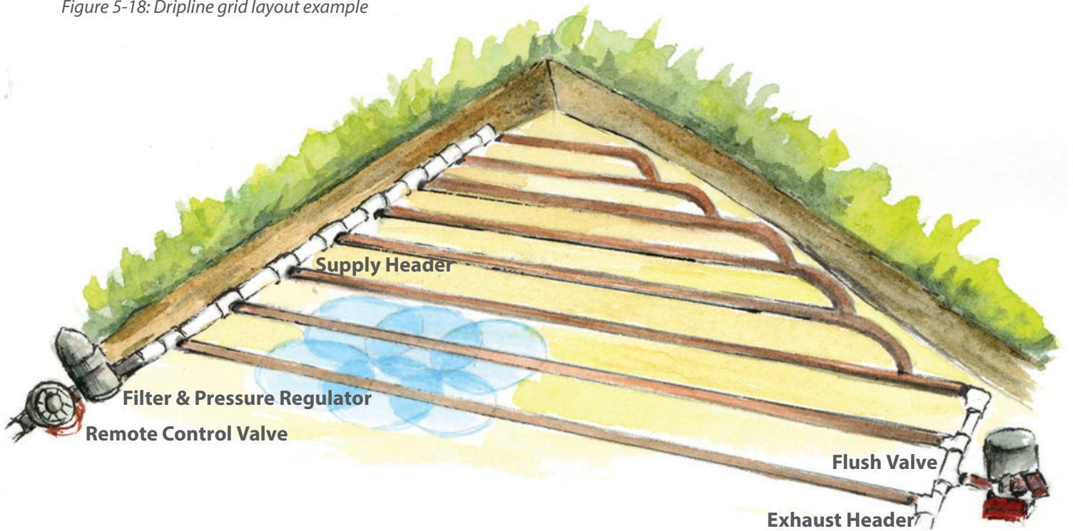
Figure 5-18: Dripline grid layout example
