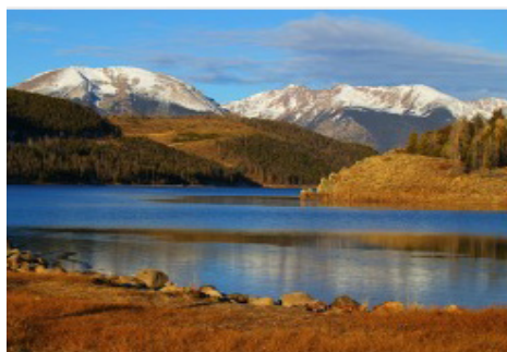
Figure 1-9: Dillon Reservoir
