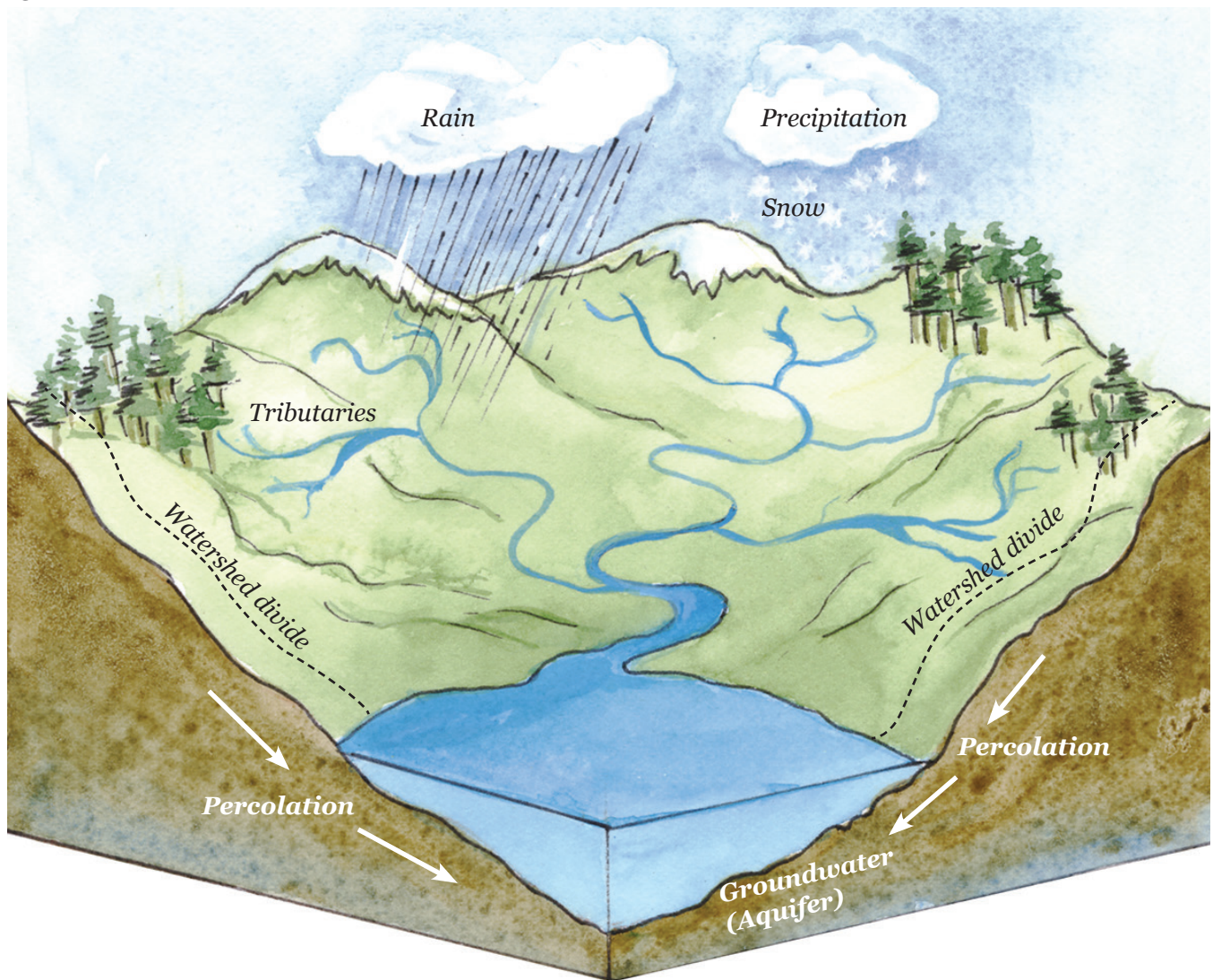
Figure 1-3: Watershed
