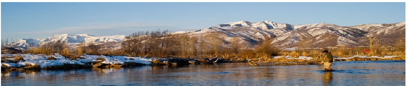
Figure 1-15: Eagle River
