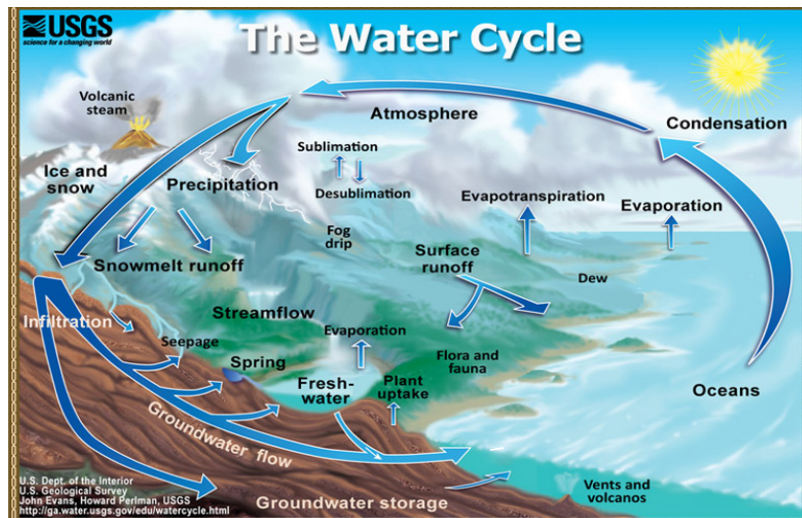
Figure 1-1: Water cycle
