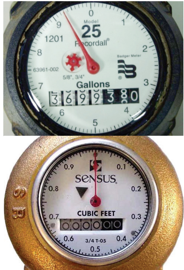
Figure 1-12: Straight-reading meters in gallons (upper) and cubic feet (lower)
