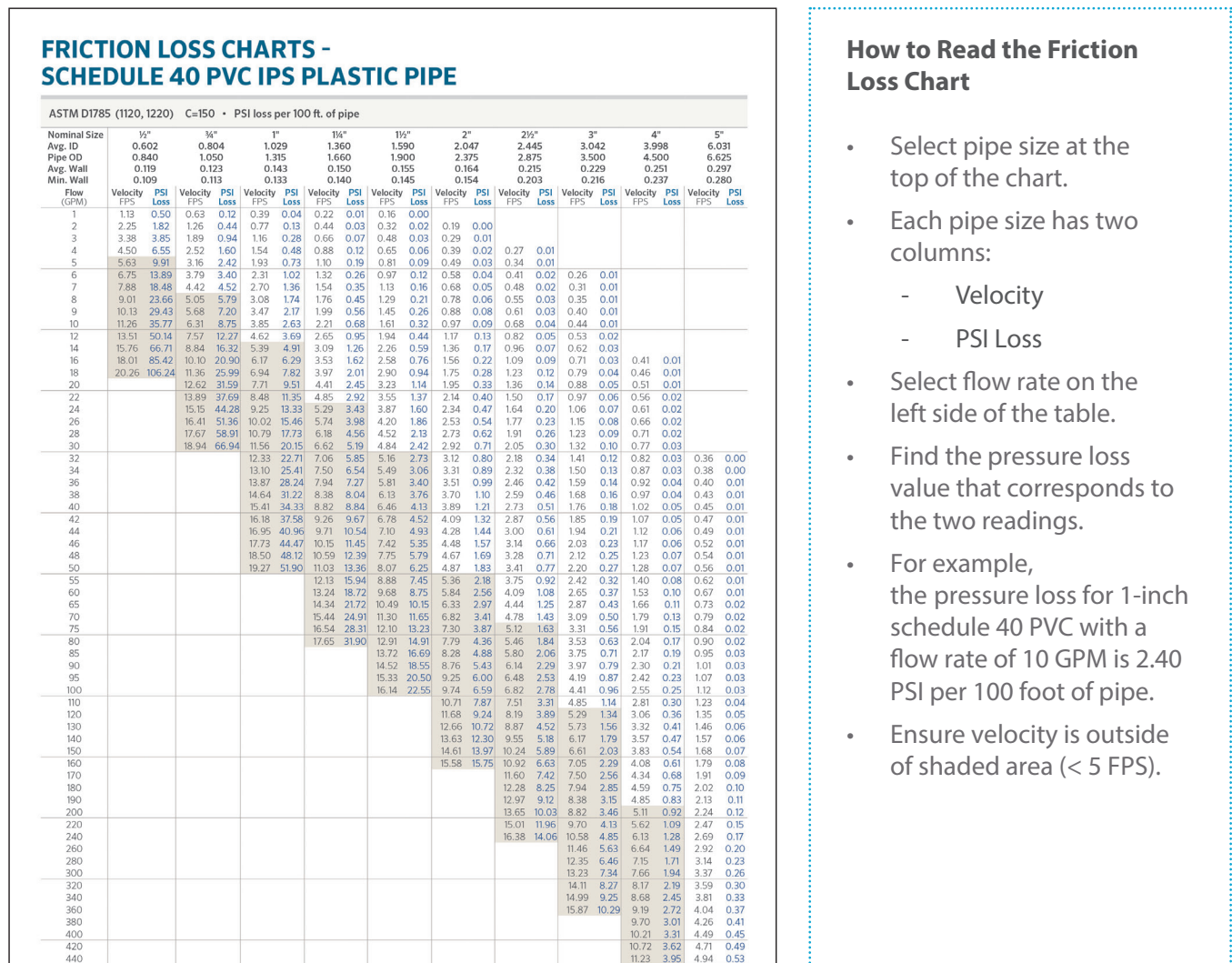
Figure 5-2: Friction loss chart for schedule 40 PVC (image courtesy of Hunter Industries Inc)
