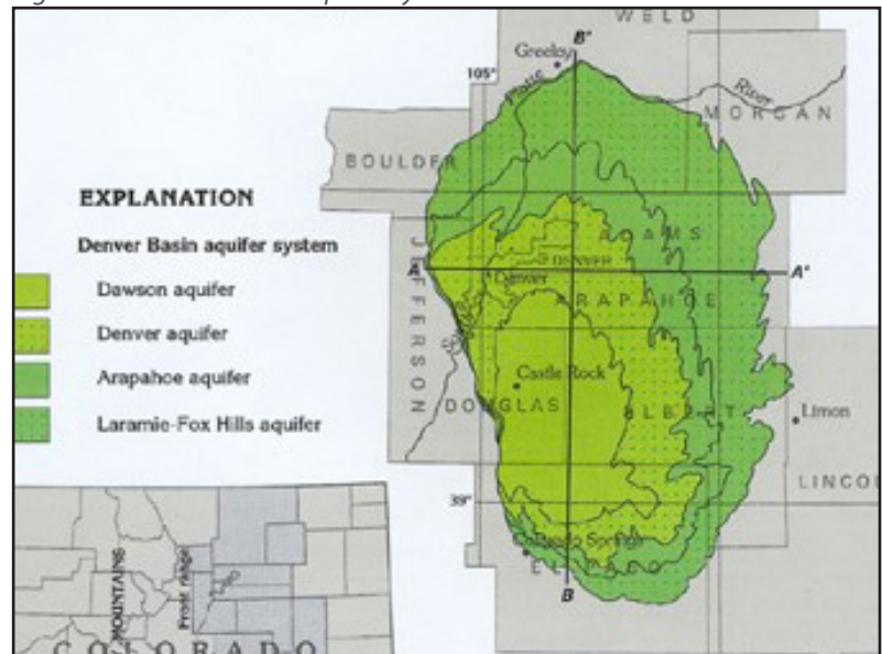
Figure 1-6: Denver Basin Aquifer System
