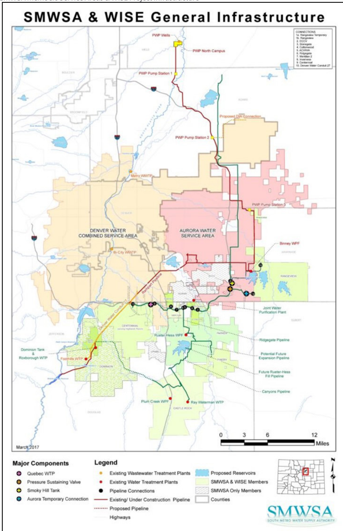
Figure 1-7: SMWSA Members Service Areas & WISE Project Infrastructure
