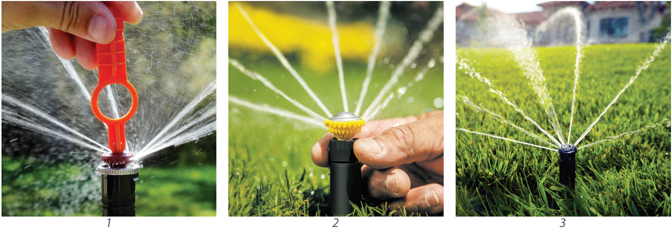
Figure 5-15: Left to right (1) Hunter MP Rotator, (2) Rain Bird R-VAN, (3) Toro Precision Series Rotating Nozzle (images courtesy of Hunter Industries Inc, Rain Bird Corporation, and The Toro Company)
