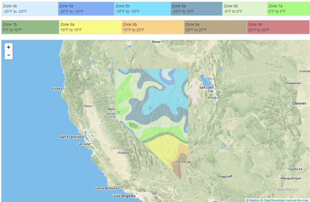
Figure 4-3: Nevada USDA Hardiness Zone Map for Nevada ( https://planthardiness.ars.usda.gov/PHZMWeb/ )
