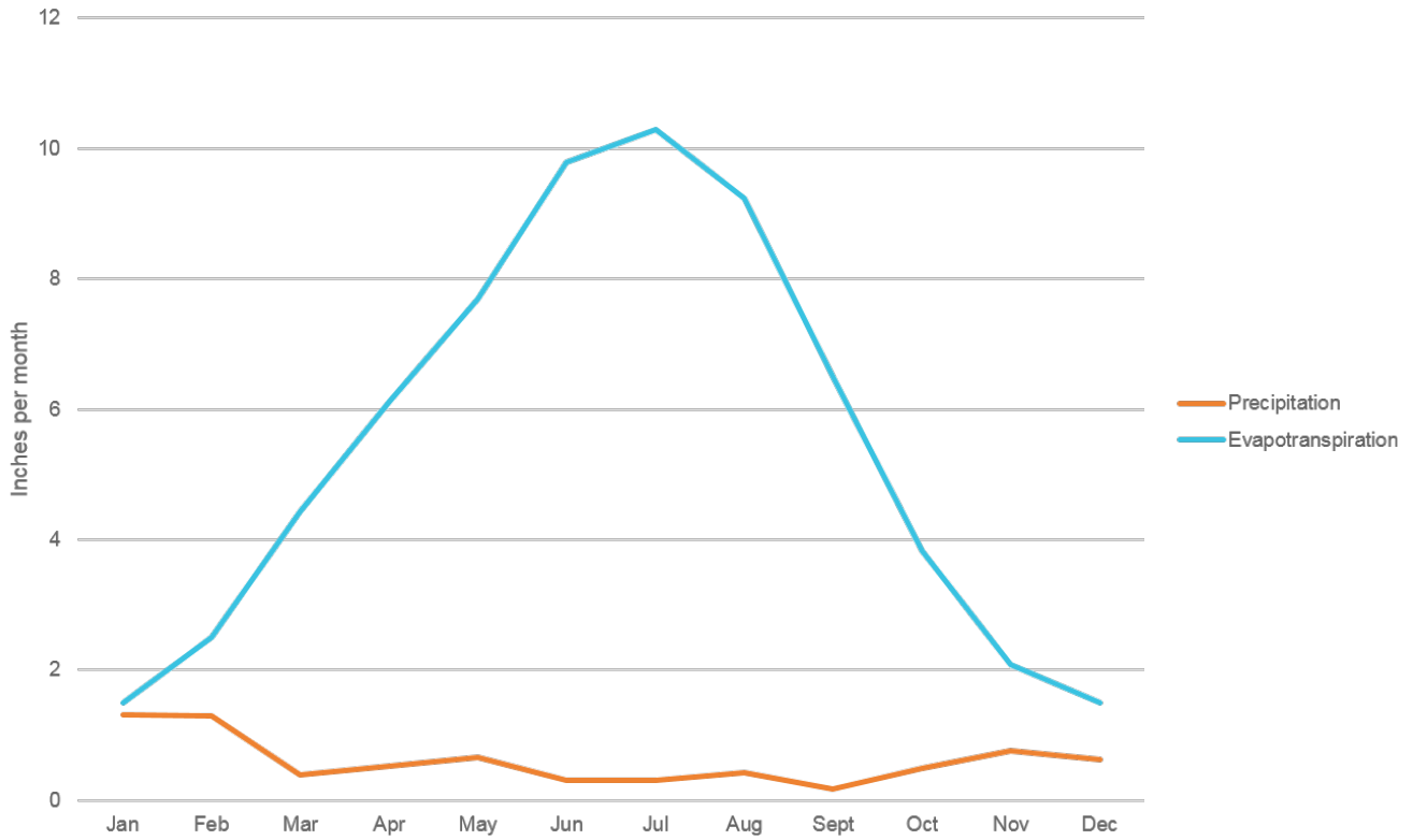
Figure 4-4: UNR Campus Precipitation and Evapotranspiration averaged over 2013-2017
