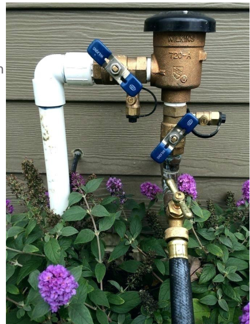
Figure 6-4: Backflow device.
