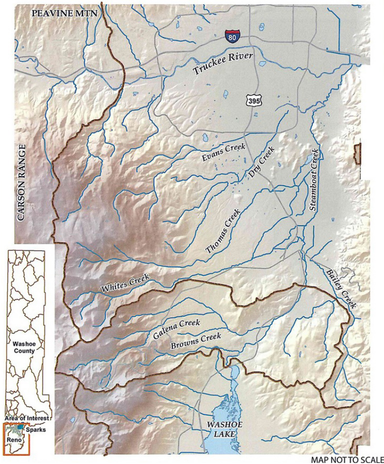
Figure 1-6: Steamboat Creek and surface water tributaries (Department of Water Resources, Washoe County)
