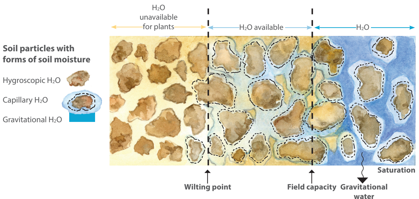
Figure 3-14: The soil moisture reservoir
