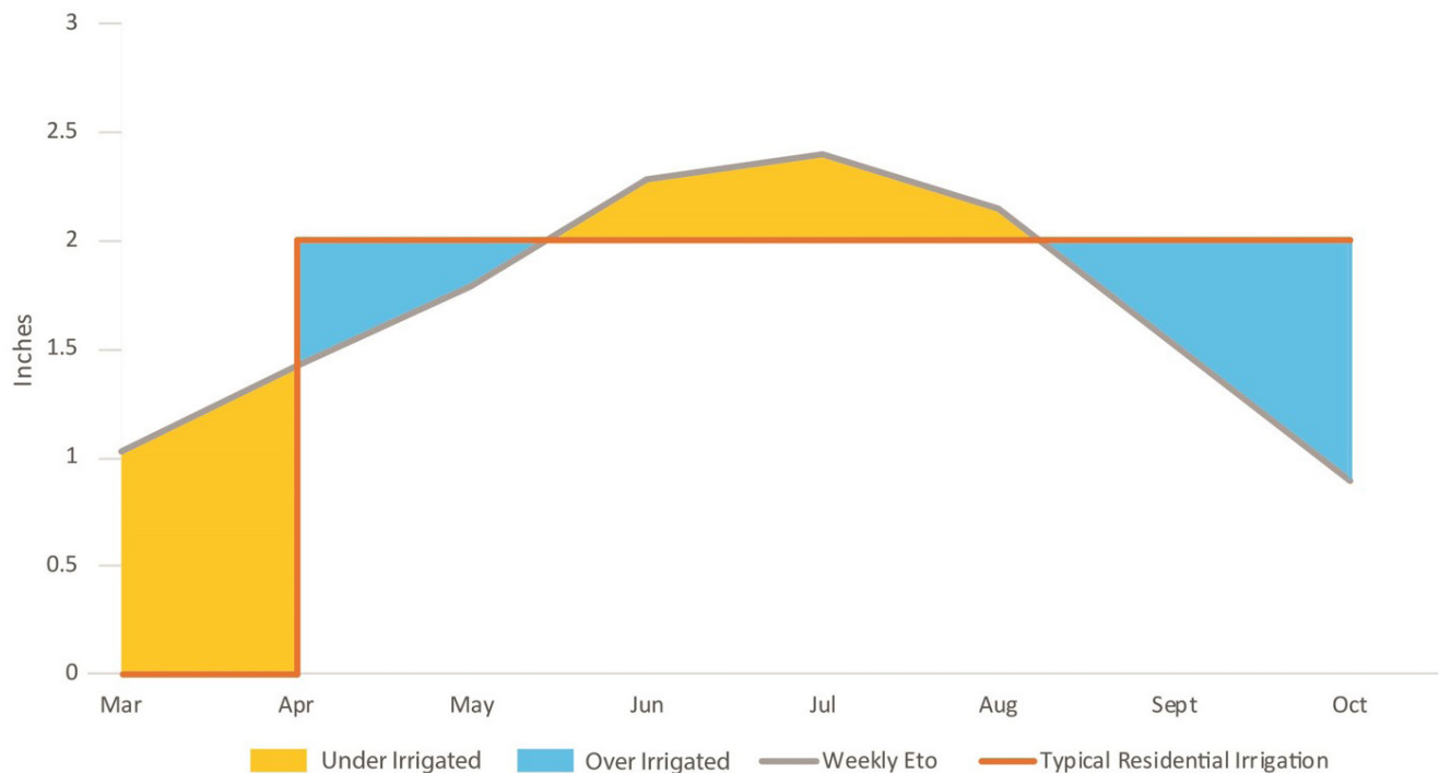
Figure 8-2: Weekly ETo for UNR Campus station vs. typical residential irrigation
