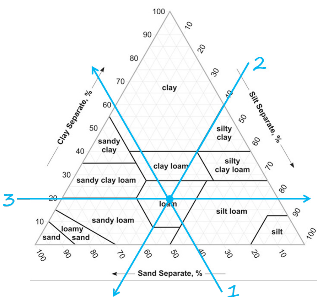
Figure 3-5: Soil textural triangle (image courtesy of United States Department of Agriculture)
