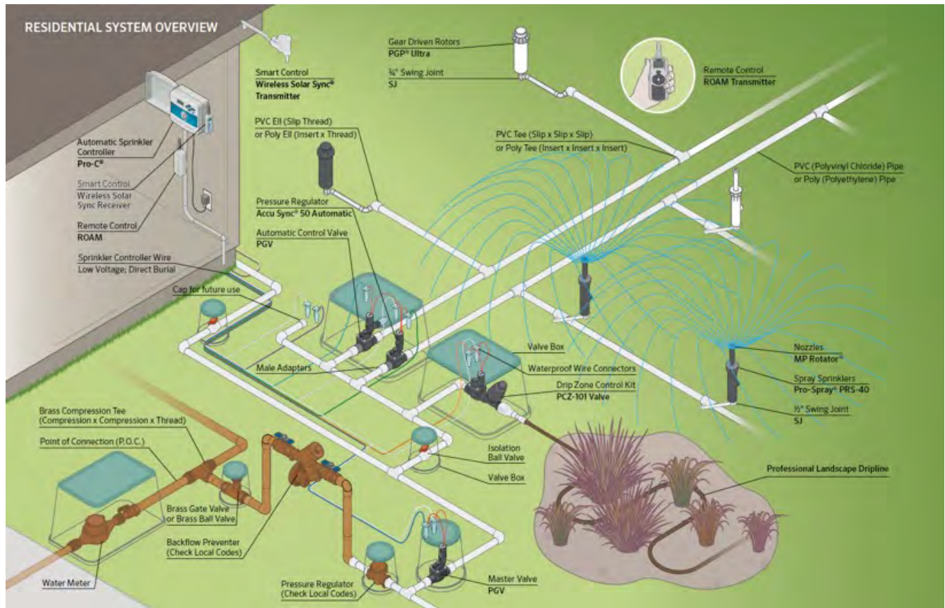
Figure 5-6: Irrigation system overview (image courtesy of Hunter Industries Inc)
