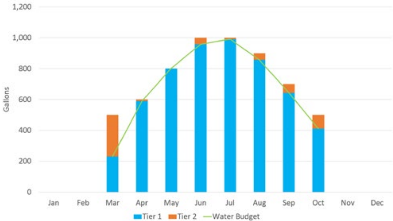
Figure 10-3: Sustainable landscape monthly water budget vs water usage
